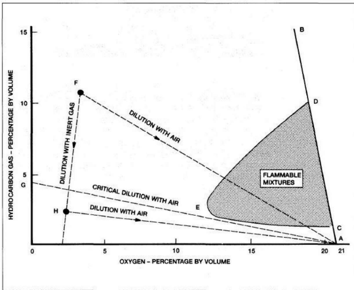
Fig. 4.1.5.B.: Flammability diagram
