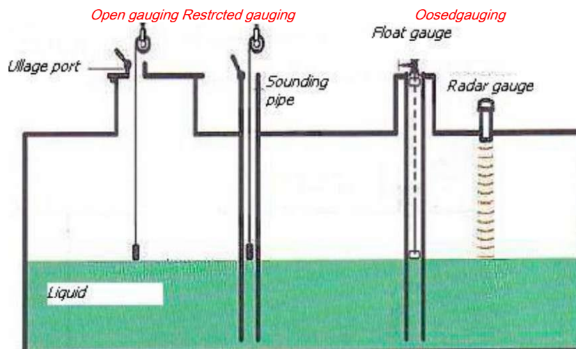
Figure : Types of gauging
