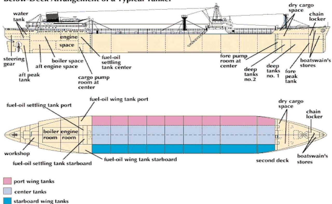
Fig. 1.2.: Basic Deck Arrangements of a Typical Tanker
