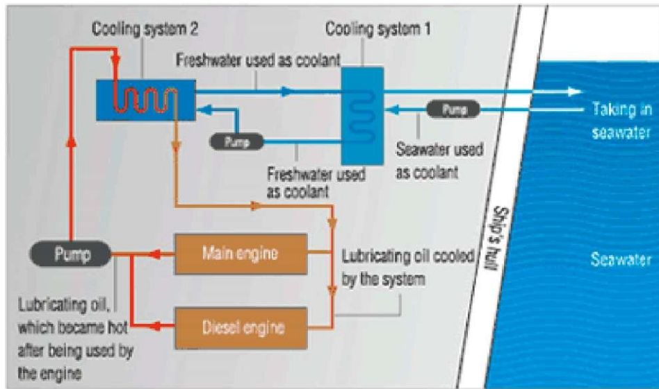
Fig. 9.2.C: Central Cooling System 9.3 SOPEP and SMPEP SOPEP
