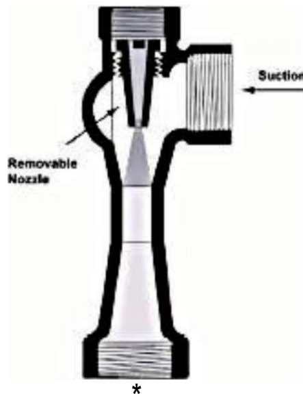
Fig. 1.4. E: Water jet eductors 17
