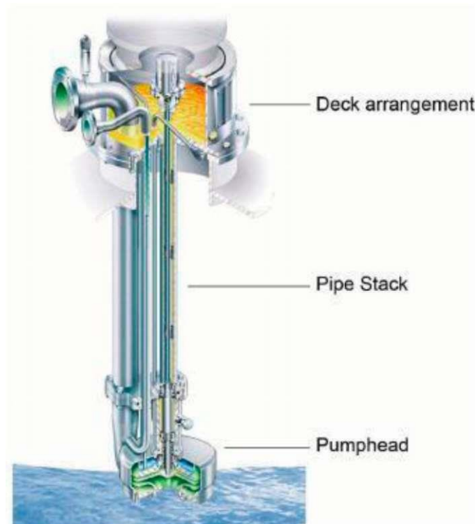
Fig. 1.4. B: Submerged pump
