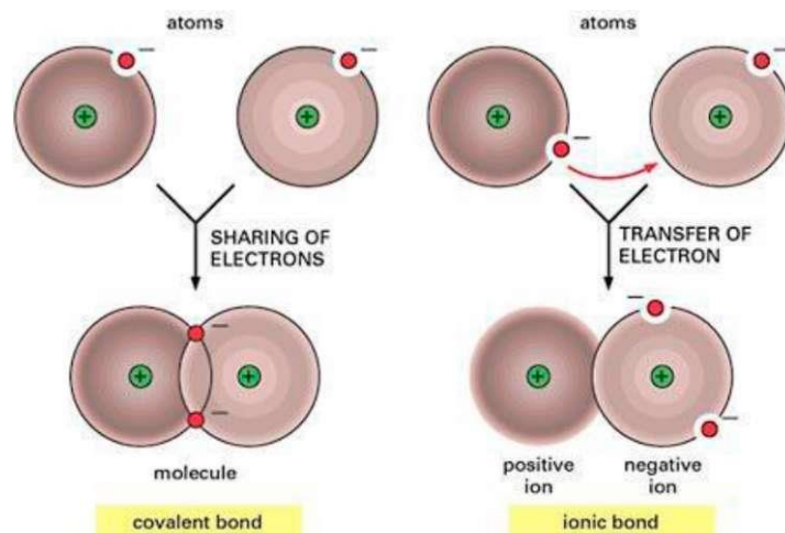
Fig. 2.2.B: Covalent Bond and Ionic bond
