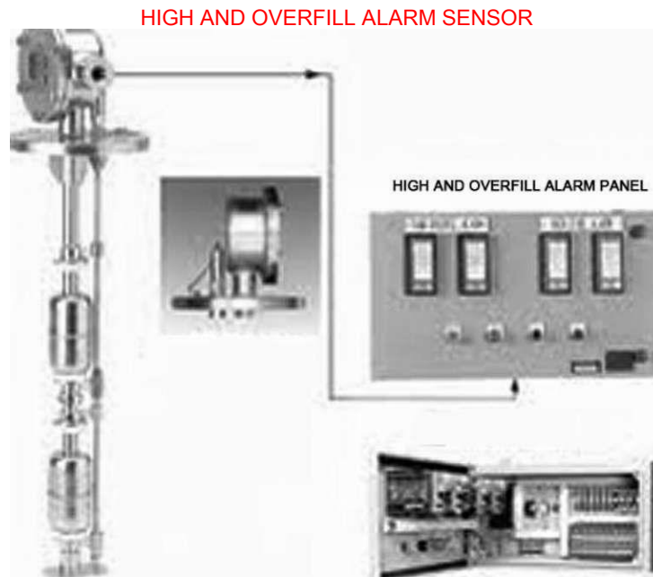
Fig. 8.3.A: High level and overflow alarms
