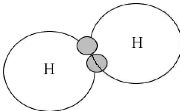
Fig. 2.2.A: Hydrogen becomes chemically stable by sharing an electron with another hydrogen atom.
