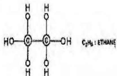
Fig. 2.2.D: Schematic representation of hydrocarbon molecules
