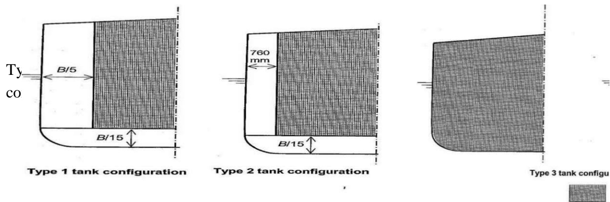
Fig. 1.3.C: Chemical Tanker Ship type configuration as per IBC Code
